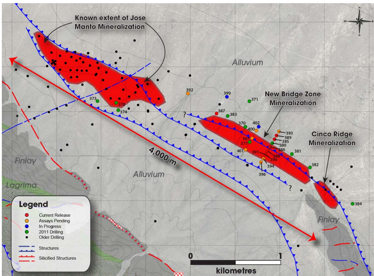
Diagram Two: Drill plan
